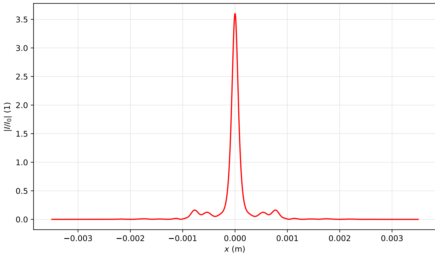
Intensity profile I(x, y = 0, z = 1.194)/I_0 , P_{in}=8.5P_{cr} , artificial time
